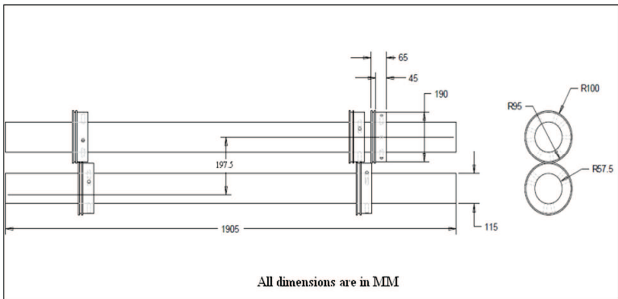
Figure 4.2 Drafting of machine components
