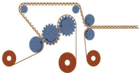
Figure 2.2: The manufacturing of a single wall corrugated board.
