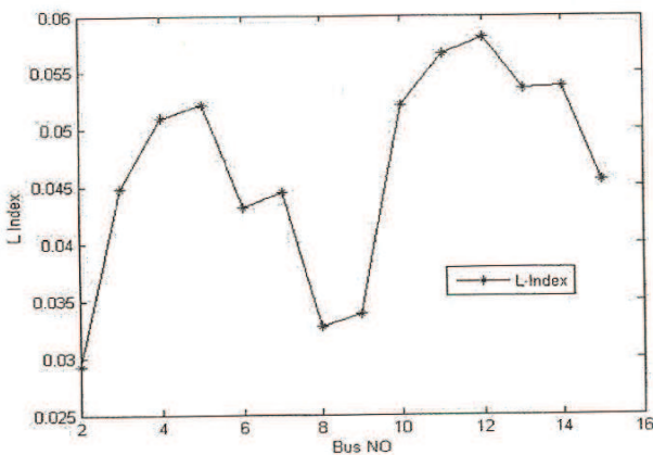
Fig. 1. L- index of 15- bus system.
