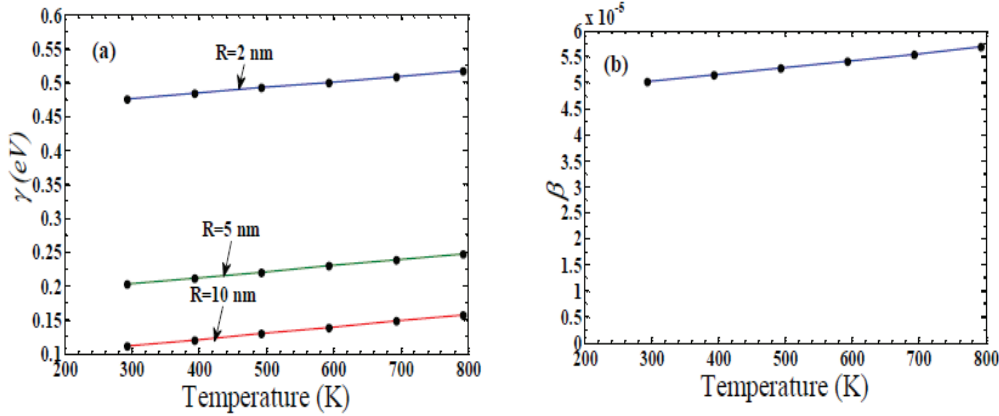
Fig. 1 (a) & (b) Variation of damping constant \gamma and volume expansion coefficient \beta of nanoparticle with Temperature
